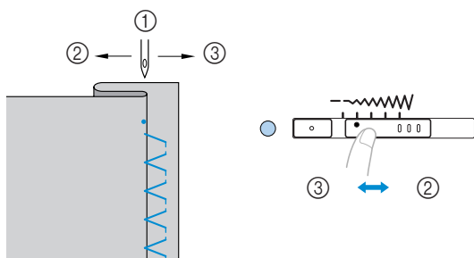
① Needle drop point ② Wider stitch ③ Narrower stitch
